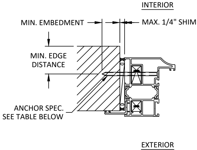
G 6 INSTALLATION DETAIL JAMB WITH FLANGE
