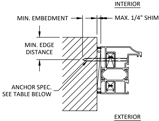
F 6 INSTALLATION DETAIL JAMB
