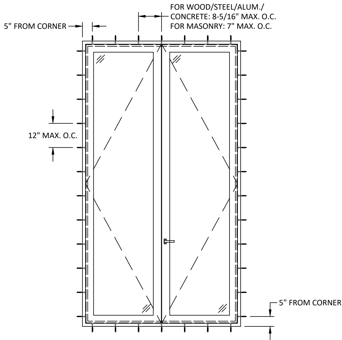
ANCHOR LAYOUT FRENCH DOOR
