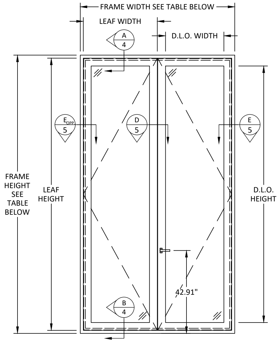
TYPICAL ELEVATION FRENCH DOOR
