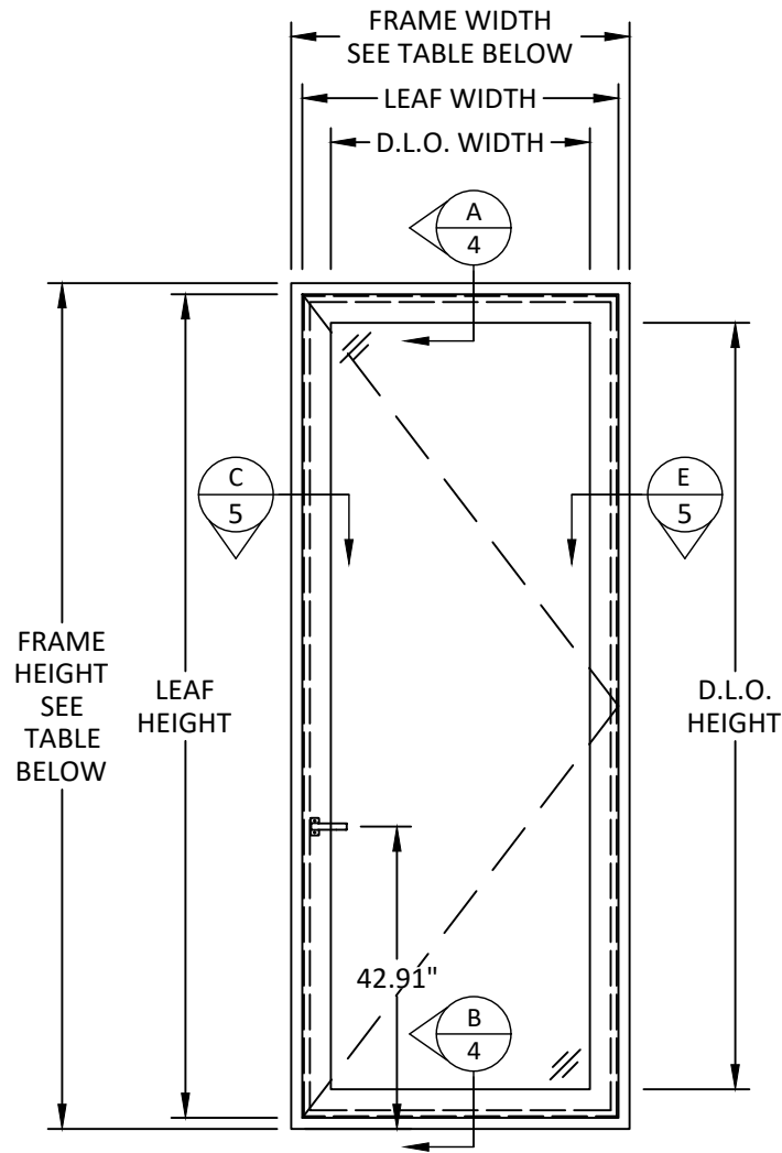
TYPICAL ELEVATION SINGLE DOOR
